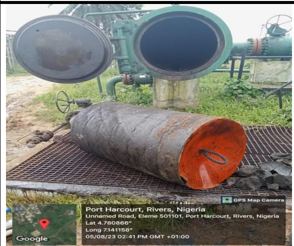
RECOVERED 28" MD BARE BODY FOAM PIG
