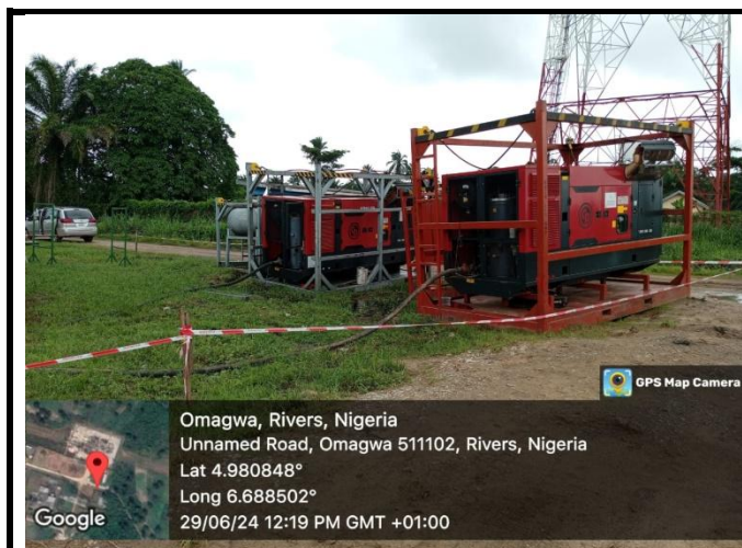
AIR COMPRESSORS USED FOR DRYING OPERATION
