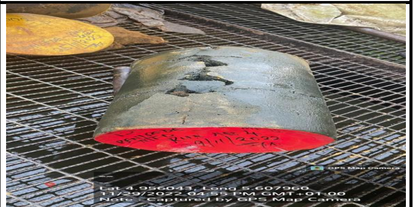
LOADED 12" MD BARE BODY FOAM PIG (RUN 7)
