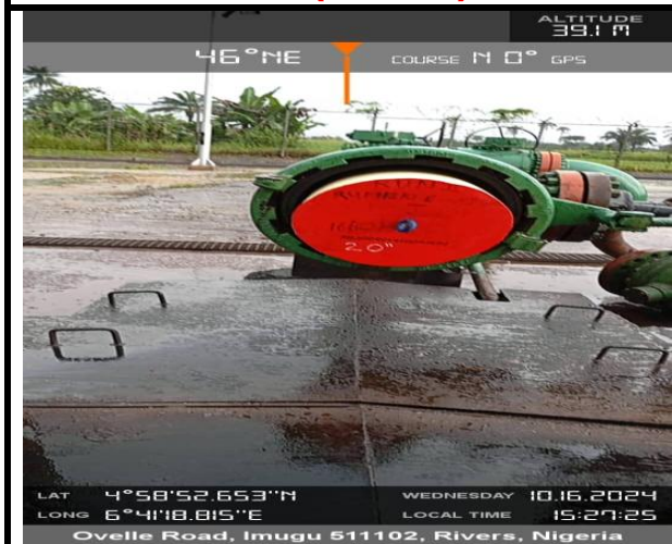
LOADED 20" MD BARE BODY FOAM PIG (RUN 1)
